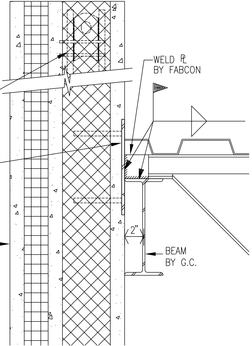
DETAIL 1 \frac{1}{2}'' = 1'-0''
